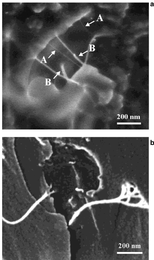
Figure 1. (a) Field emission SEM images of CNTs- C_{16}H_{32}O_2 -epoxy composite for 0.8 wt % CNTs and 1:1 CNTs to C_{16}H_{32}O_2 weight ratio. The arrows indicate (A) individual CNTs and (B) CNTs covered with palmitic acid. (b) Field emission SEM images of CNTs-epoxy composite for 0.8 wt % CNTs without palmitic acid. The scale bar corresponds to 200 nm.
